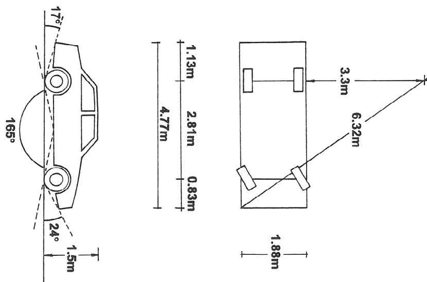
90% Design Motorcar Scale 1:100
