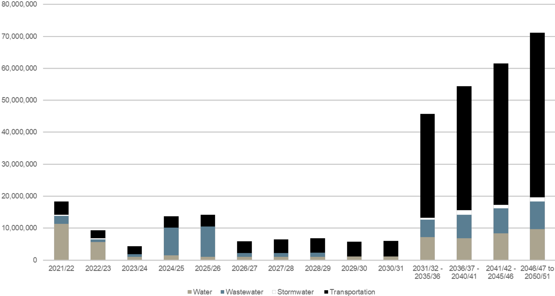
Figure 22: Projected Capital Expenditure - Infrastructure Assets (Inflated)
