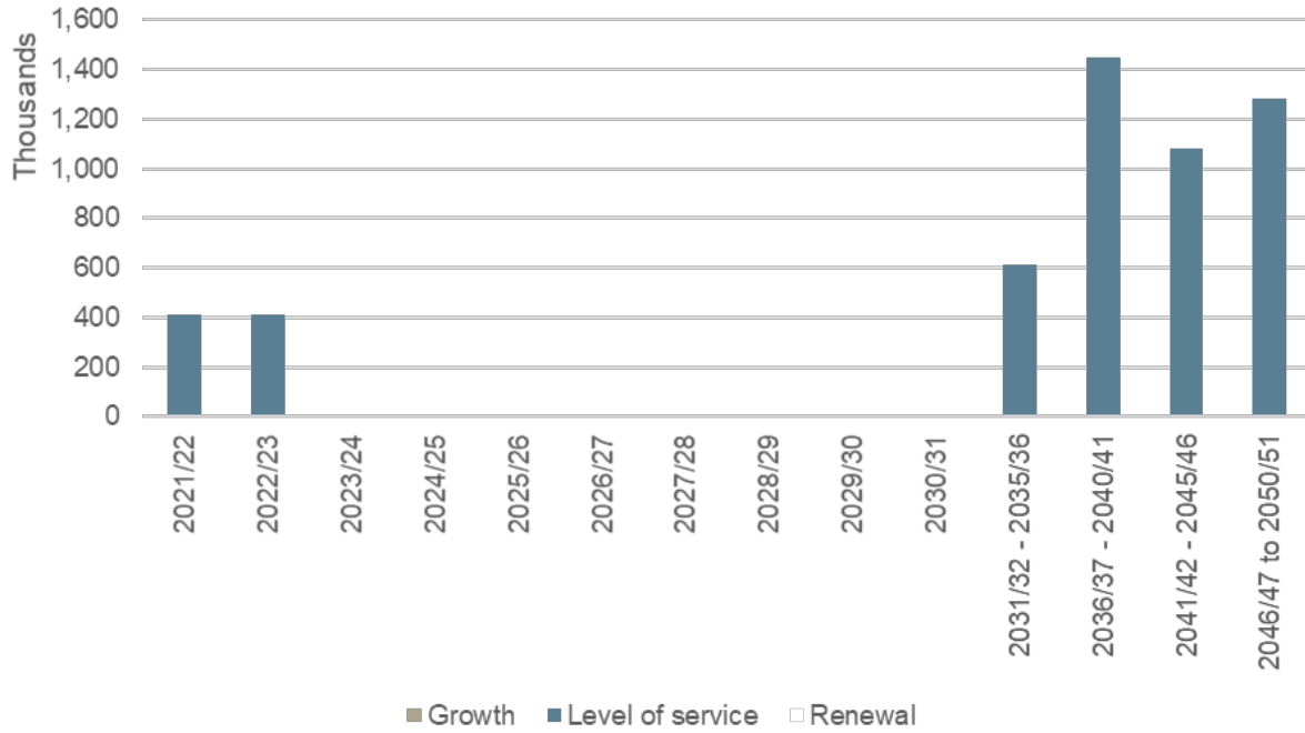
Figure 18: Stormwater Projects Cost Profile (Inflated)
